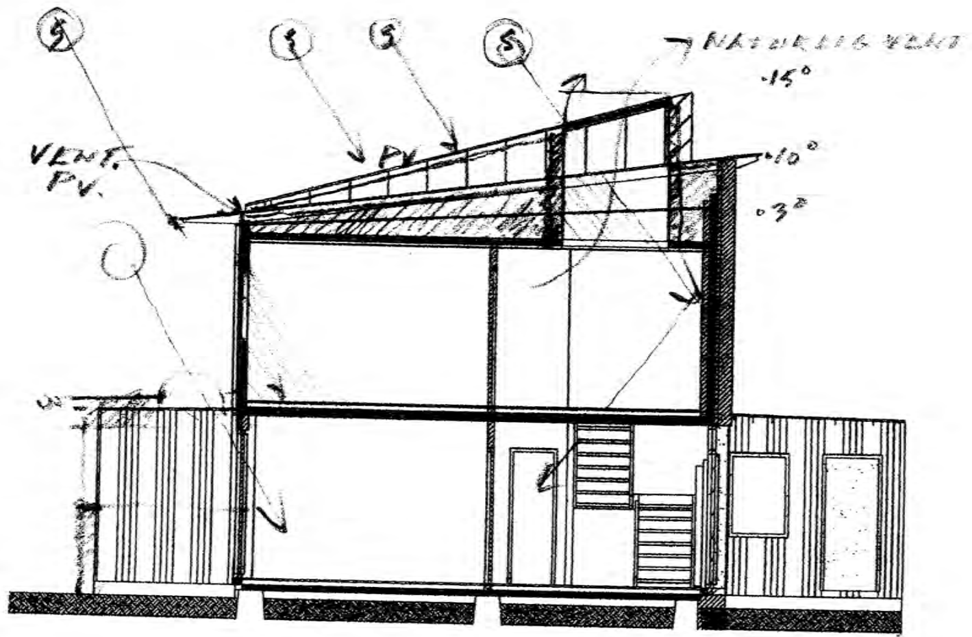
CROSS SECTION WITH PV TAGS + OVERLAYS
